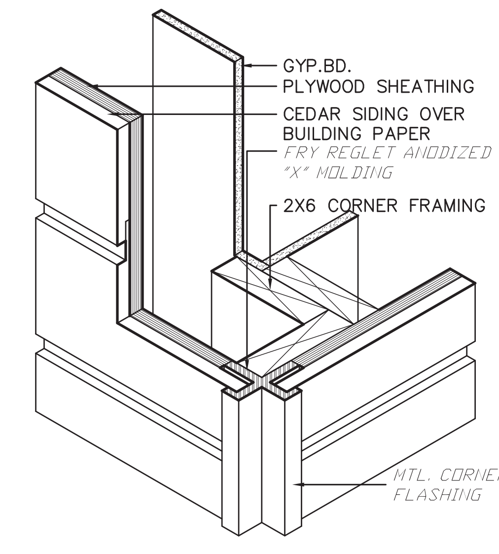
4 WOOD SIDING CORNER DETAIL 3" = 1'-0"
