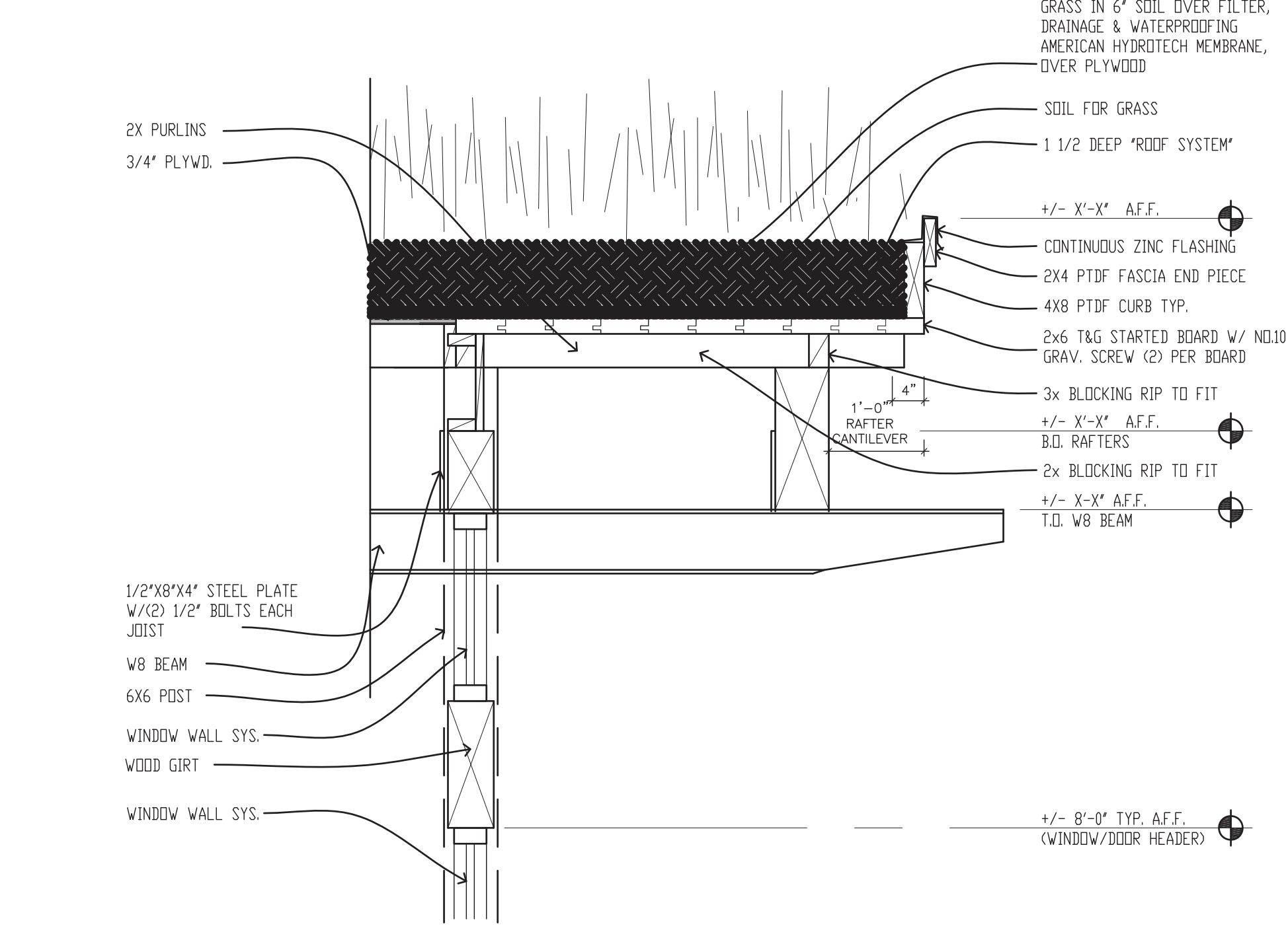
8 RAKE DETAIL 3/4" = 1'-0"
