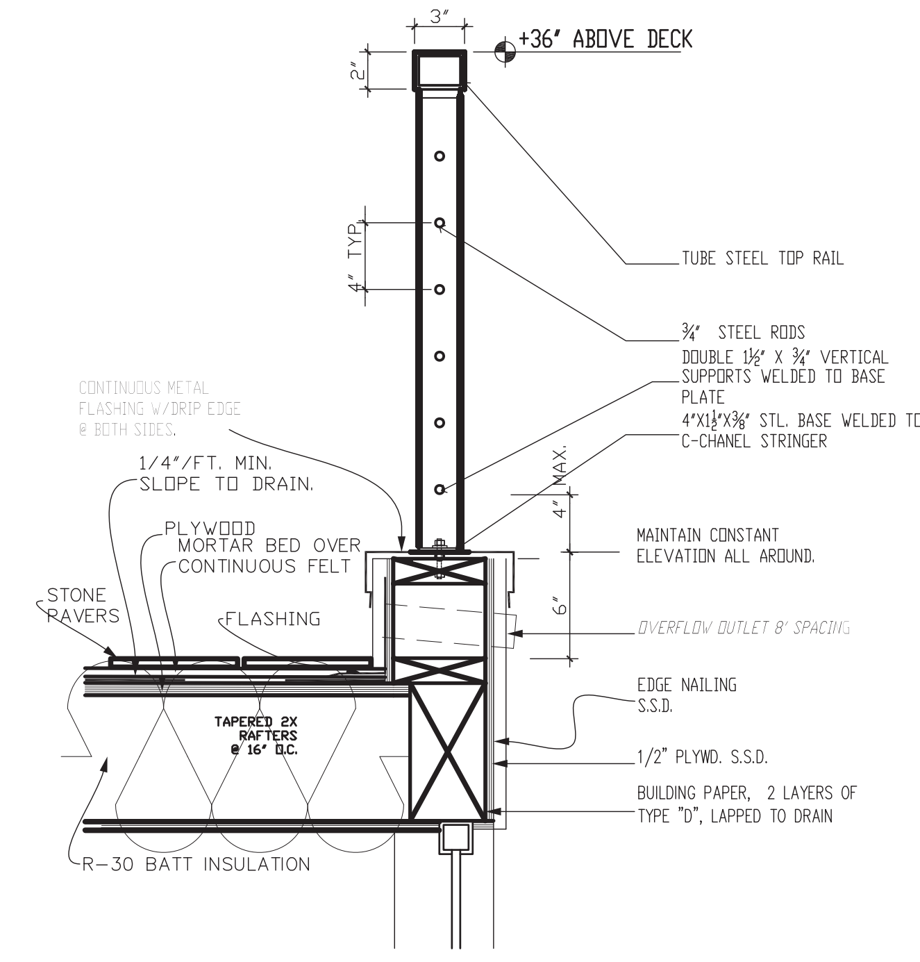
9.1 HANDRAIL RAIL BOARD DETAIL - ELEVATION 1 1/2" = 1'-0"
