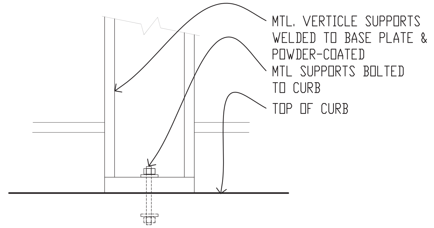
9.3 BASE DETAIL @ DINING FLOOR 3" = 1'-0"
