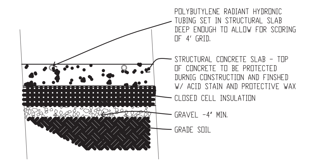
3 RADIANT HEAT SLAB 3/4" = 1'-0"
