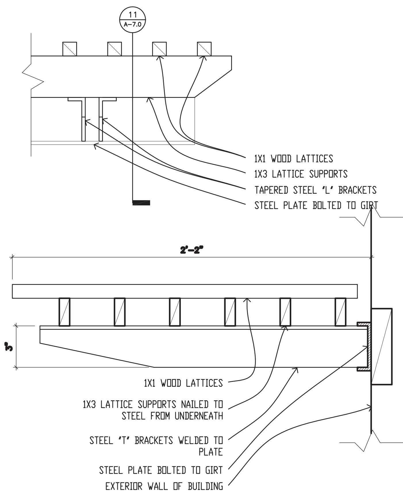
11 SUN SHADE DETAILS 3" = 1'-0"
