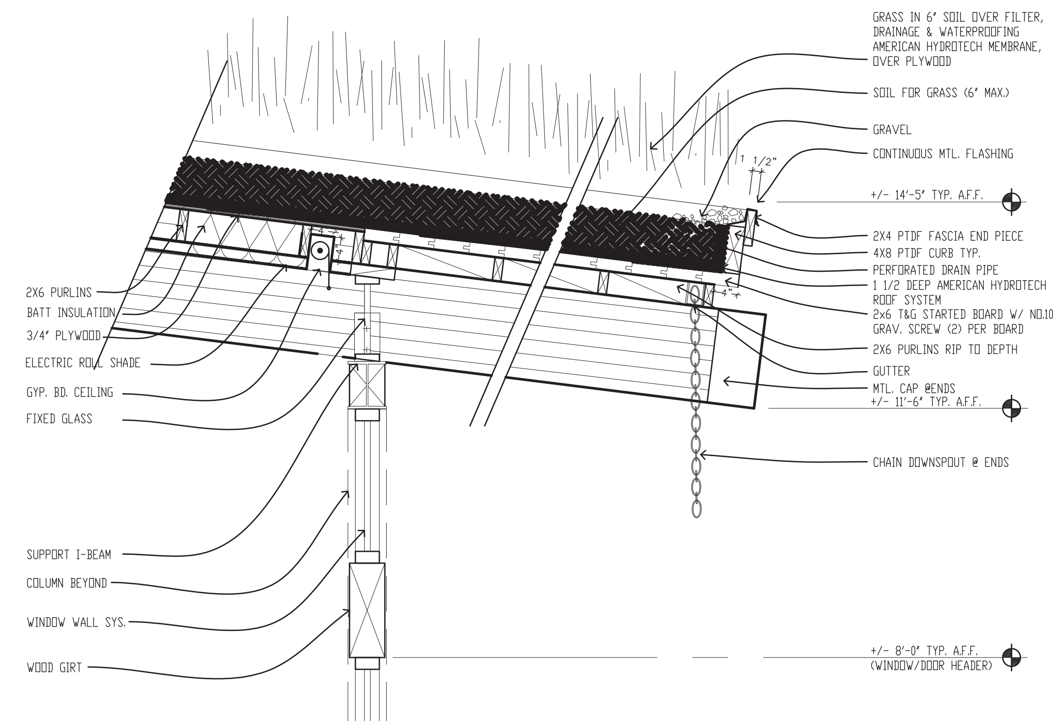
7 EAVE DETAIL 3/4" = 1'-0"
