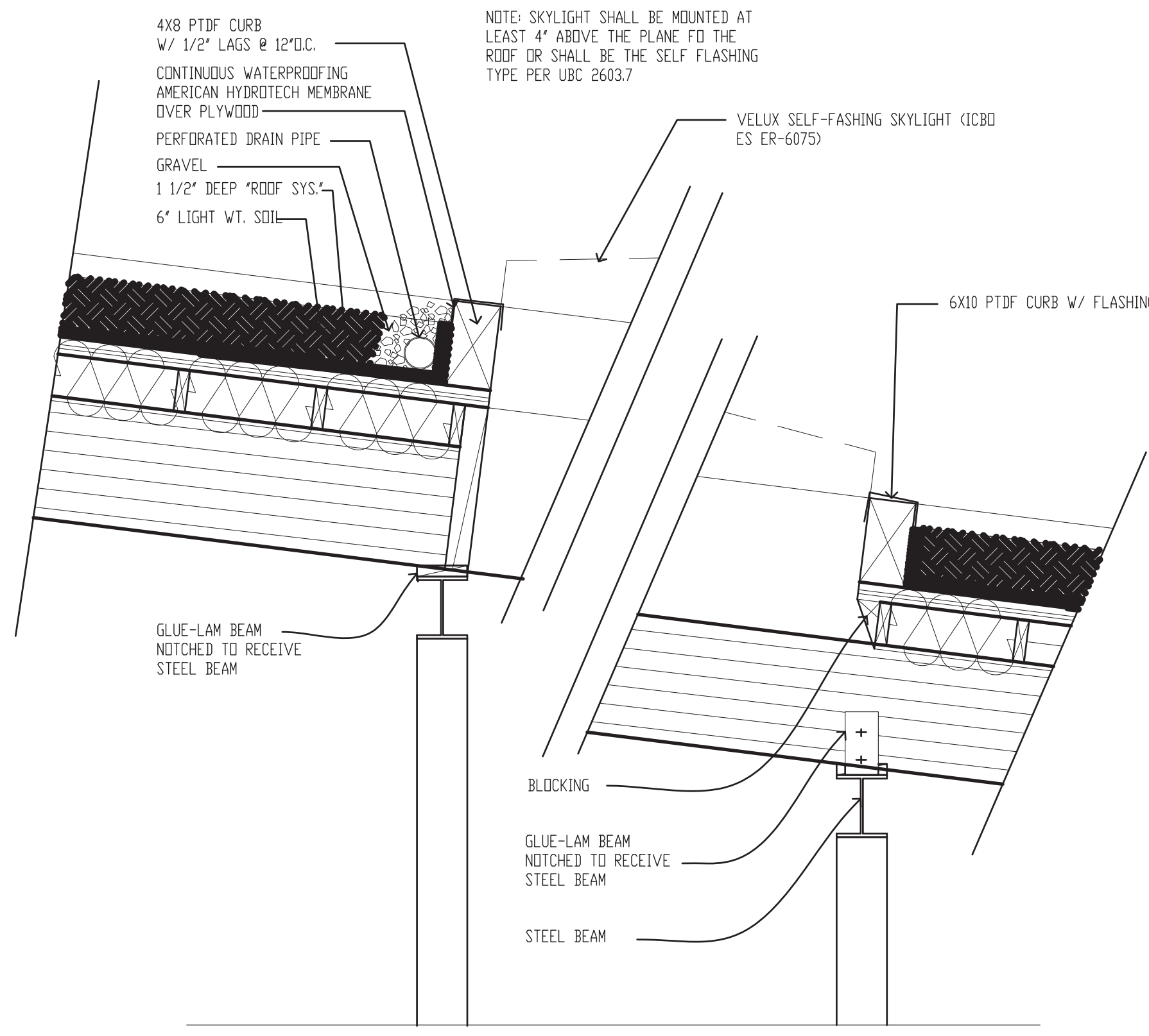
6 SKYLIGHT DETAIL 3/4" = 1'-0"
