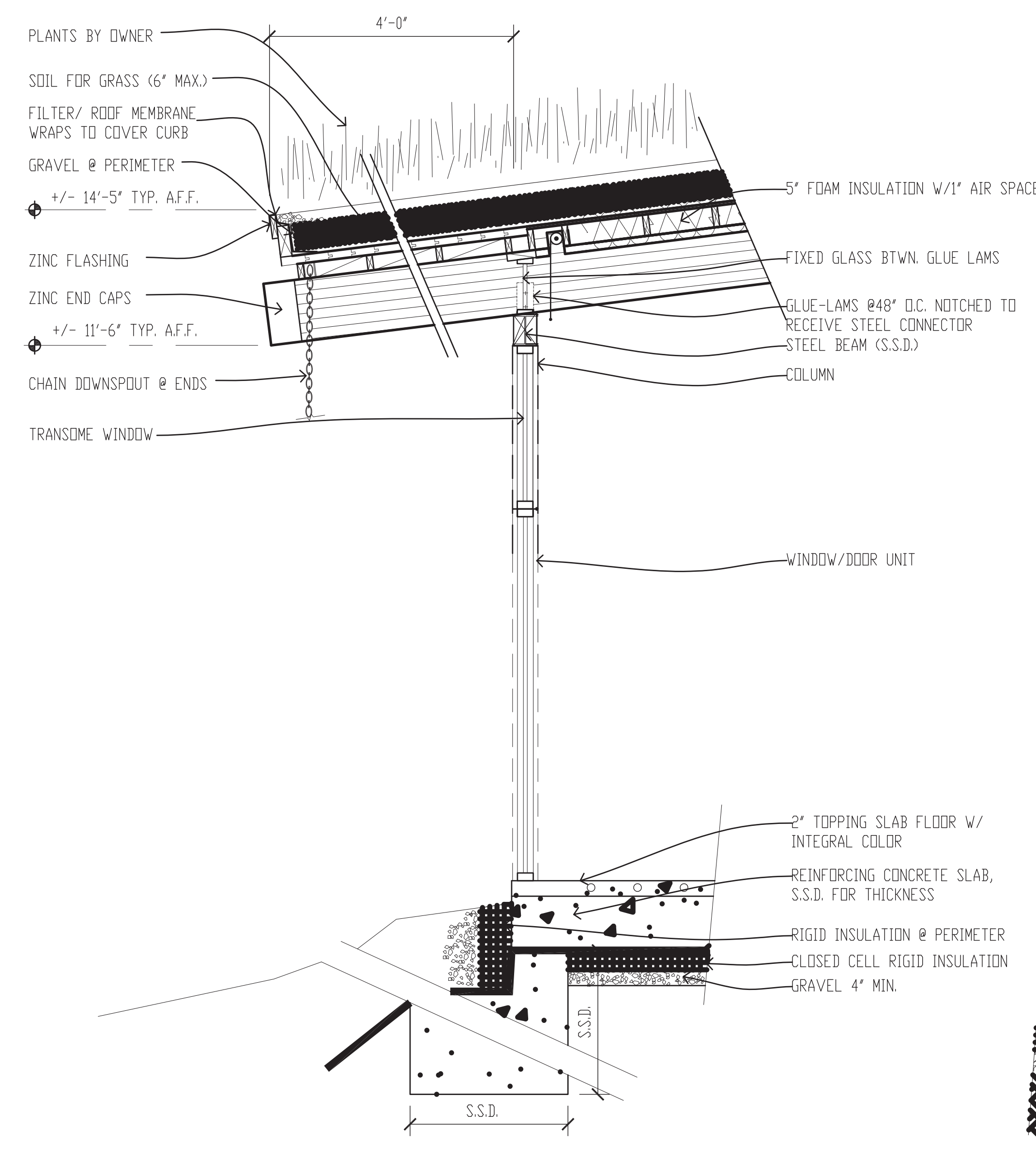
2 WINDOW WALL SECTION @ LIVING ROOM 1 1/2" = 1'-0"
