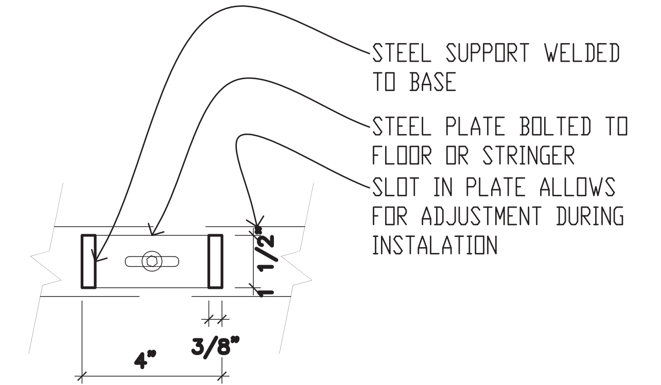
9.2 RAIL SUPPORT, TYP 3" = 1'-0"
