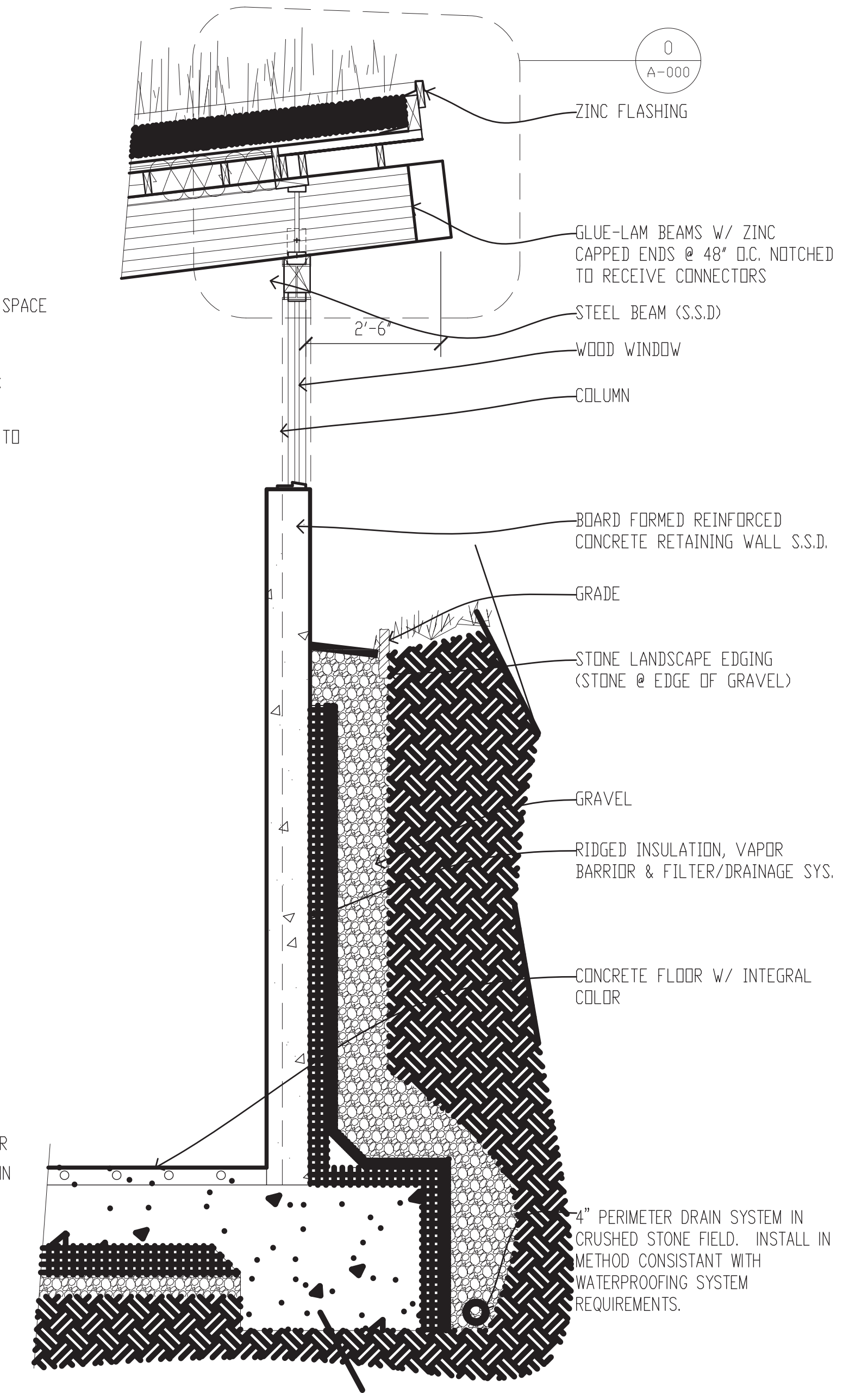
1 RETAINING WALL SECTION @ LIVING ROOM 1 1/2" = 1'-0"
